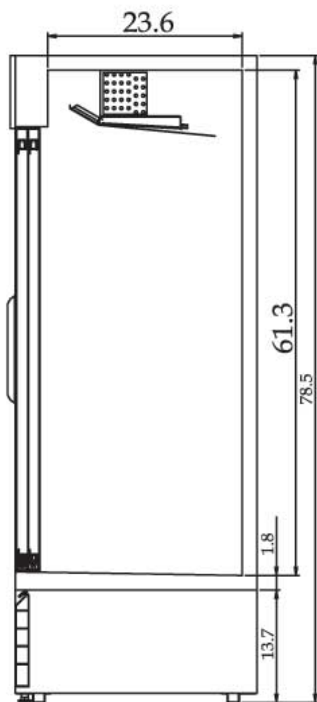
TGM-35R/48R SIDE VIEW
