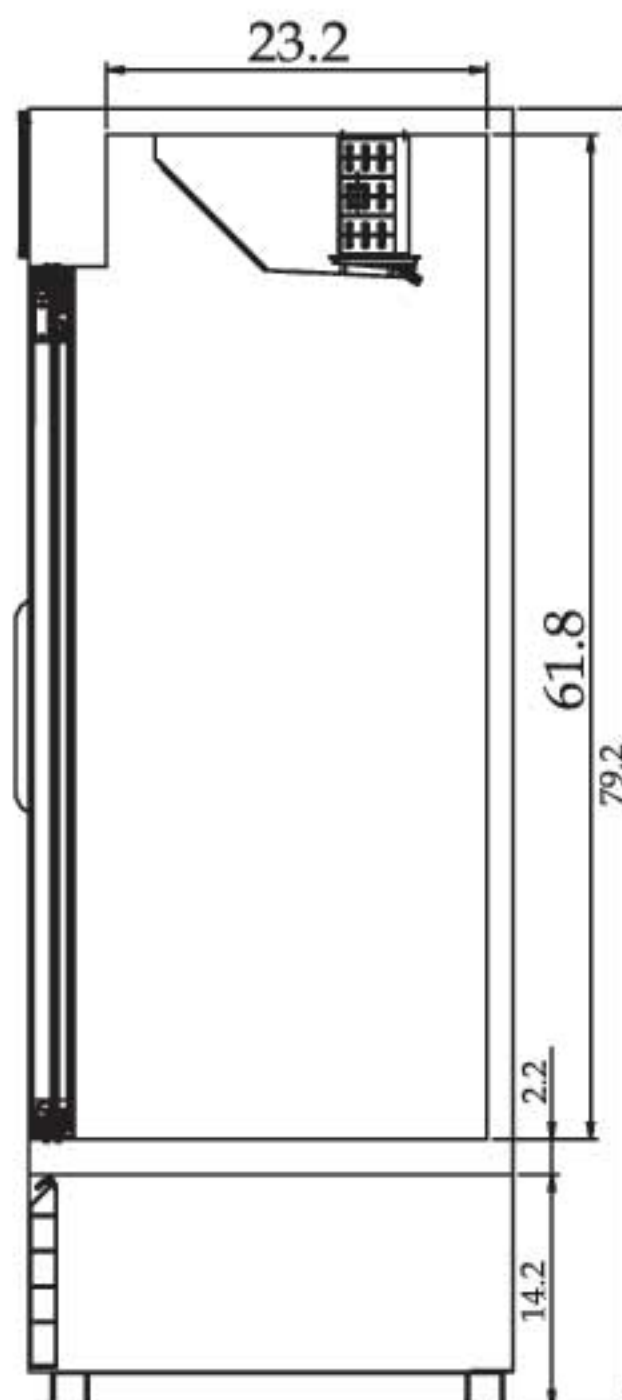
TGM-69R SIDE VIEW
