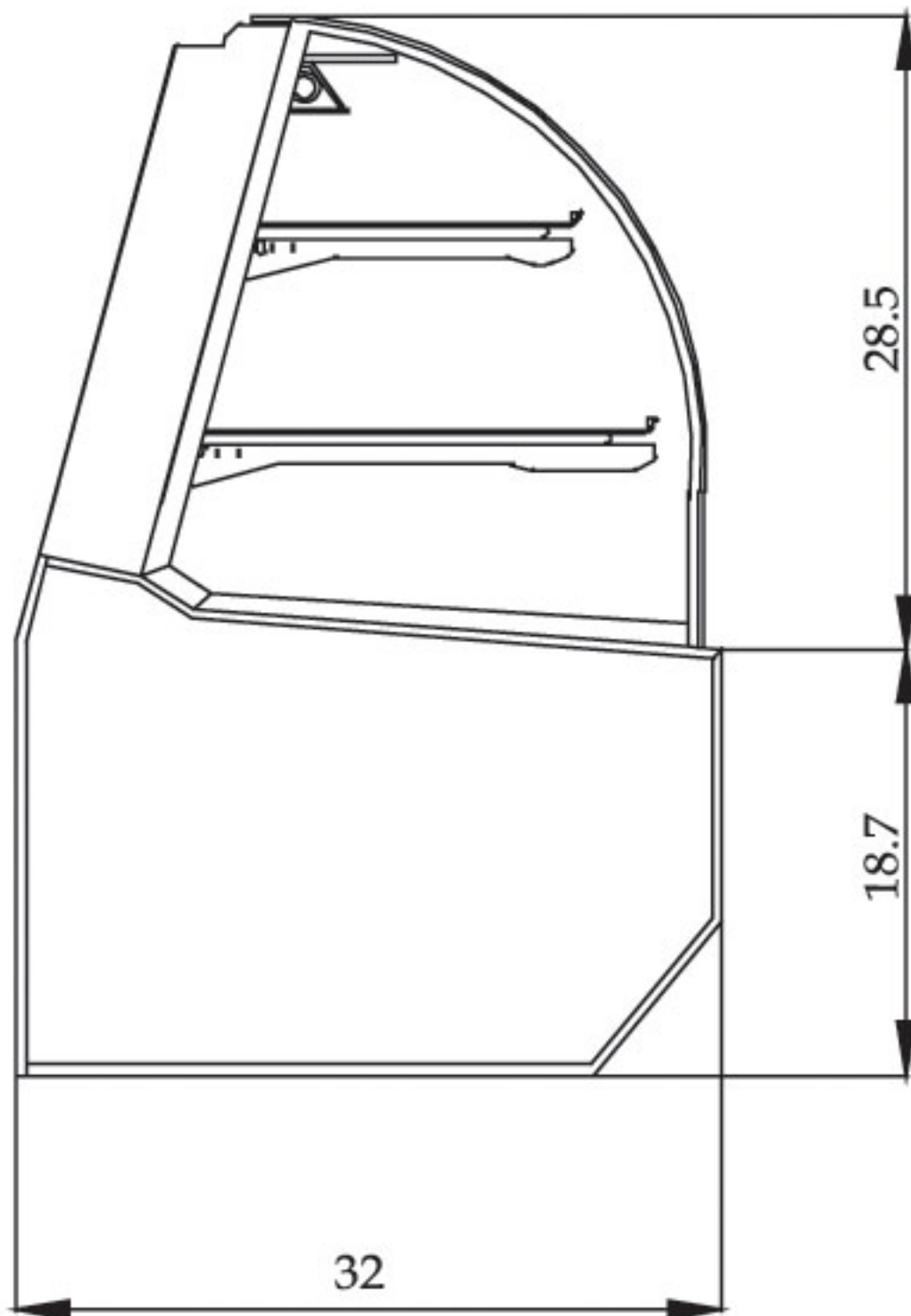
TD-4R/TD-5R SIDE VIEW
