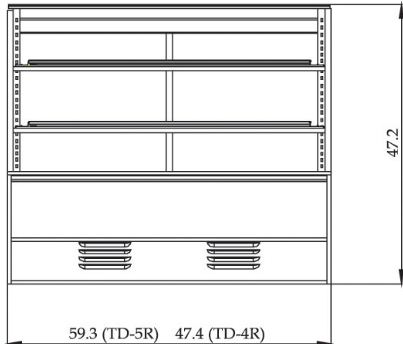
TD-4R/TD-5R FRONT VIEW
