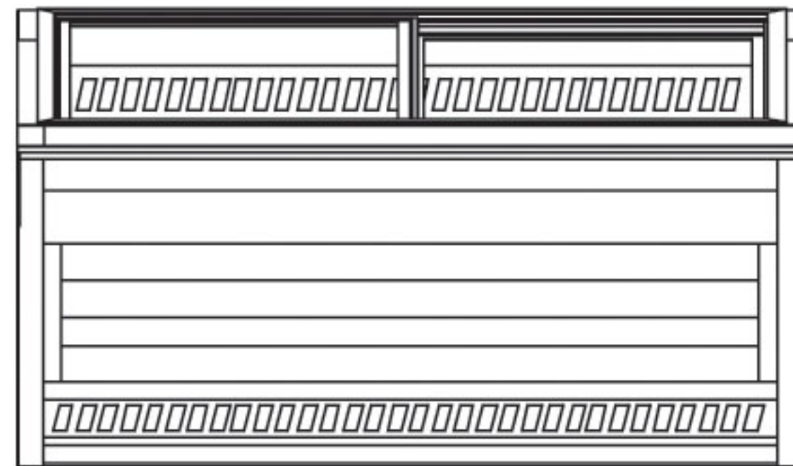
TD-4R/TD-5R PLAN VIEW
